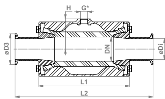
Exempl. view (DN 65 – DN 100)
