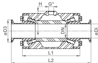
Exempl. view (DN 10 – DN 50)
