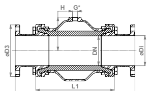
Exempl. view (DN 65 – DN 100)
