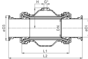
Exempl. view (DN 65 – DN 100)
