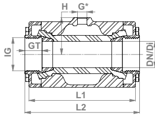
Exempl. view (DN 10 – DN 50)
